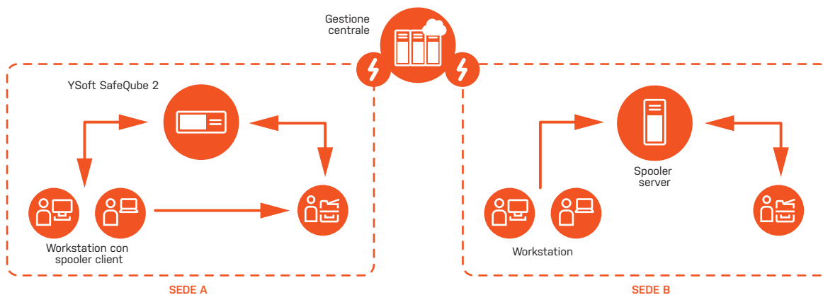
Figura 3. Client Based Print Roaming con YSoft SafeQube 2 facoltativo
